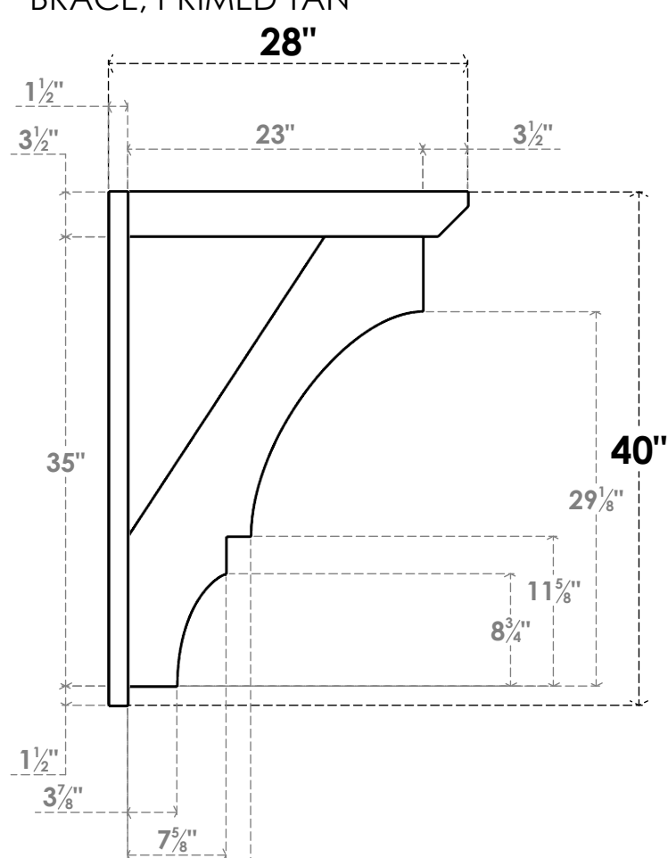
SIDE PROFILE
